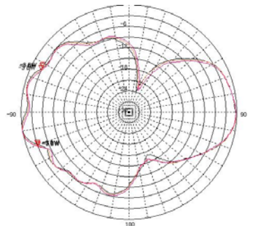
Vertical Pattern
